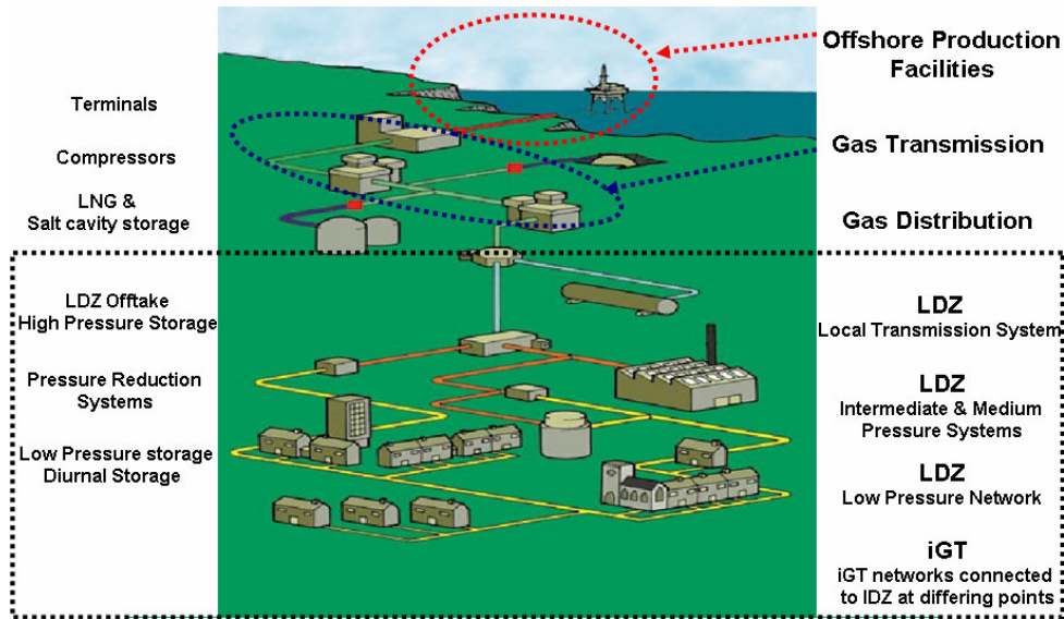
Figure 2.1 Directional Flow of Gas
