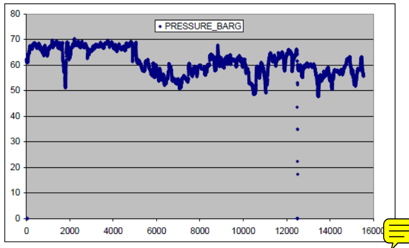
Figure 5.1 – SMER Period Pressure Change
