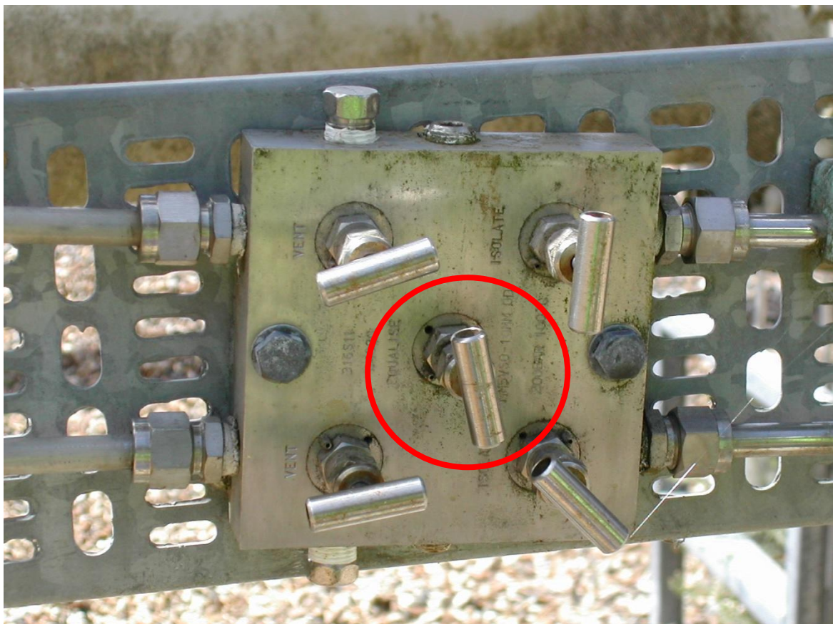
Figure 3.4 – Common \Delta P Isolation Manifold
